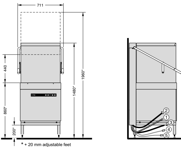
Hood-type dishwasher model 602
