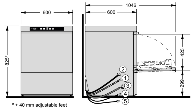
Undercounter dishwasher model F503
