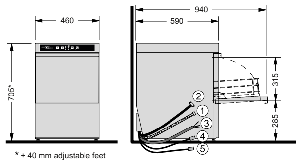
Glasswasher model G403
