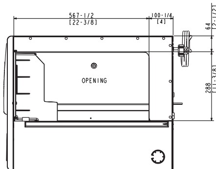
Base View
